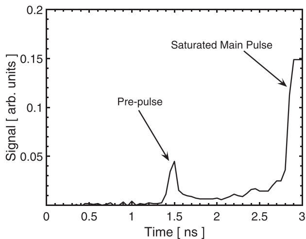
FIG. 1. Example raw data from the watercell diagnostic from one shot ( \tau_{\text{Laser}} = 2.9 \text{ ps} , E_{\text{Laser}} = 151 \text{ J} , I = 4.6 \times 10^{18} \text{ W/cm}^2 ) on the Titan laser from this campaign. These watercell measurements were performed on-shot, thus the main laser pulse is saturated on the trace since it has such a high energy and the detector does not have the dynamic range to capture both the full main pulse signal and lower energy prepulse. To calibrate this detector, several low energy shots at millijoule energies were taken to relate the signal from the diode to an energy.
