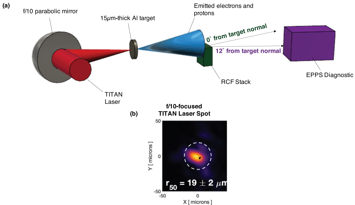
FIG. 2. The full experimental setup used in this campaign is shown in (a). The Titan laser was focused using an f/10 parabolic mirror onto a 15- \mu\text{m} thick aluminum target. The main diagnostics were a radiochromic film stack (RCF) and the electron–positron–proton spectrometer (EPPS). The RCF stack provided measurements of the TNSA proton energies and was placed at 0^\circ relative to the normal of the target, while the EPPS was used to measure the electron spectra and was placed 12^\circ from the target normal. The aluminum target was irradiated at an angle of 31^\circ relative to the laser axis. The RCF stack was placed 3.5 cm from the target rear surface and the EPPS diagnostic was 70 cm from the target rear surface. In (b), the Titan beam spot (focused with the f/10 parabola) is shown as measured on a low energy, un-amplified pulse. The dashed line shows the radius at which 50% of the energy is contained in the spot.
