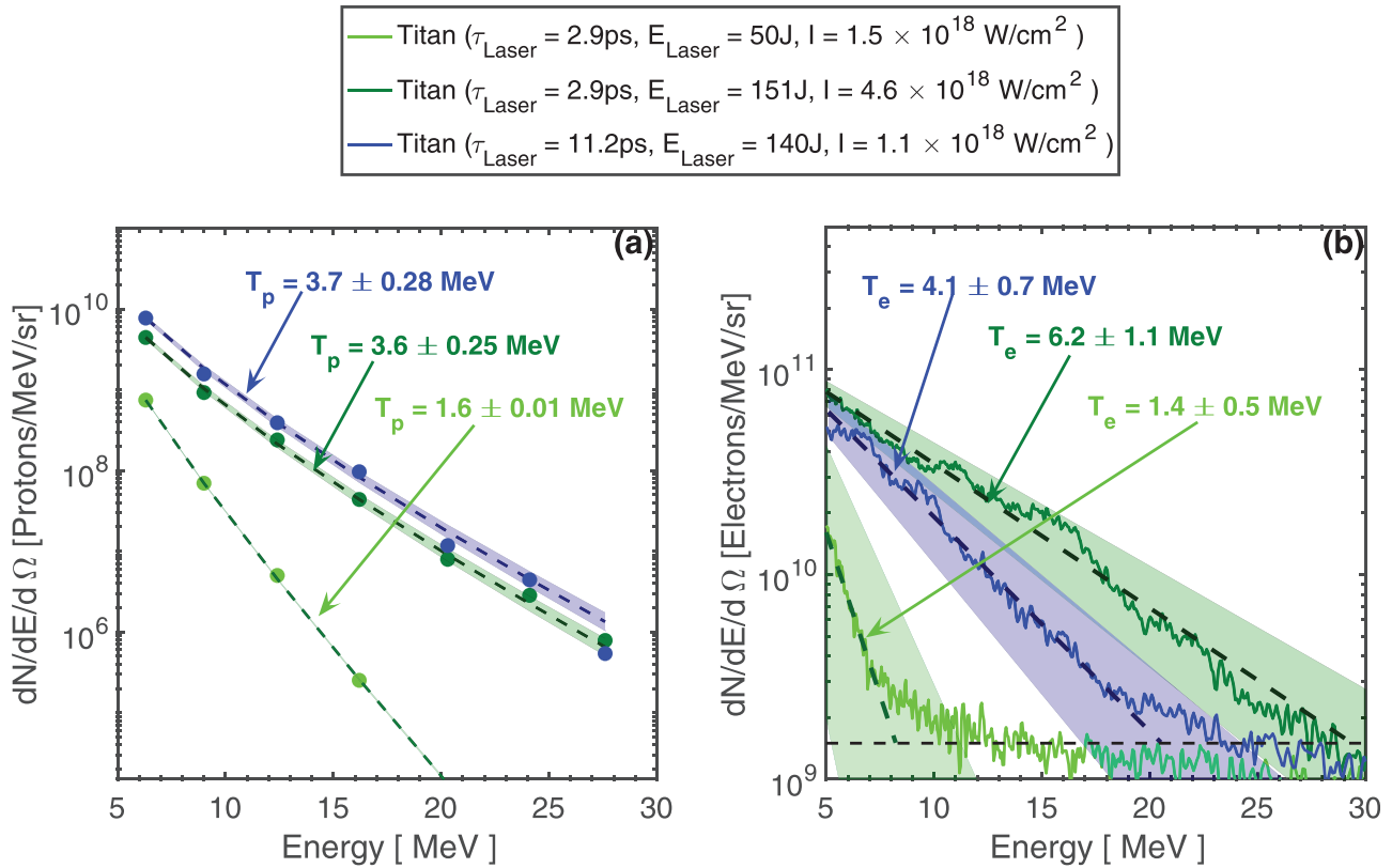
FIG. 3. (a) shows example proton spectra from the RCF stack diagnostic for three shots: a short pulse duration, high-energy shot (shown in the dark green, \tau_{\text{Laser}} = 2.9 ps, E_{\text{Laser}} = 151 J), a short pulse duration, low-energy shot (shown in light green, \tau_{\text{Laser}} = 2.9 ps, E_{\text{Laser}} = 50 J), and a long-pulse-duration, high energy shot (shown in the dark blue, \tau_{\text{Laser}} = 11.2 ps, E_{\text{Laser}} = 140 J). The shaded area for all curves in (a) represents the error in the slope temperature fit. Similarly, (b) shows the electron spectra as measured by the EPPS diagnostic for the same three shots. The shaded region represents the error in the slope temperature fit for the electron measurements. 33 For both the electron spectra and RCF spectra, the slope temperature derived from fitting the spectra with an exponential curve, shows that energy and not intensity has a dominant effect on the temperature regardless of pulse duration.
