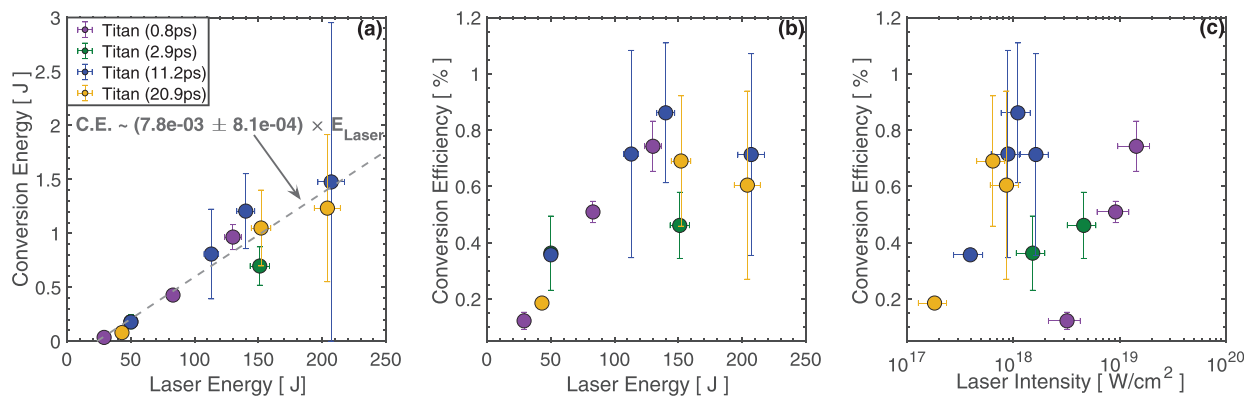
FIG. 7. The total energy into protons >1 MeV is plotted as a function of laser energy in (a). Conversion efficiency (for protons with energies >1 MeV) as a function of laser energy is shown in (b) and conversion efficiency (for protons with energies >1 MeV) is shown as a function of laser intensity in (c).
