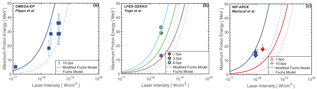
FIG. 9. (a)–(c) Shows the modified Fuchs model being applied to previous TNSA proton datasets taken on OMEGA-EP, LFX-GEKKO, and NIF-ARC.
