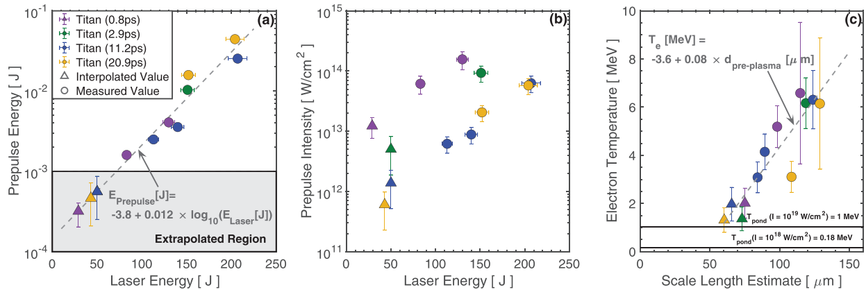
FIG. 5. Panel (a) shows the prepulse energy for all shots in this campaign. A subset of shots with main pulse laser energies below \sim 50 J had prepulse signals below the noise floor and thus these shots have extrapolated values for the prepulse energy, which are shown in triangular points instead of circular points. The relationship between prepulse energy for each shot and the main laser energy is also shown in the dashed black curve, showing that the prepulse energy depends strongly with the main laser energy for each shot. Panel (b) shows the prepulse intensity as a function of main pulse laser energy and (c) shows the electron temperature as function of the inferred plasma scale length. Overlaid on this plot in solid black lines are the value of the ponderomotive temperature given by Eq. (1) for intensities of 10^{18} and 10^{19} W/cm 2 . As the preplasma scale length decreases, we would expect the temperature to approach the ponderomotive scaling.
